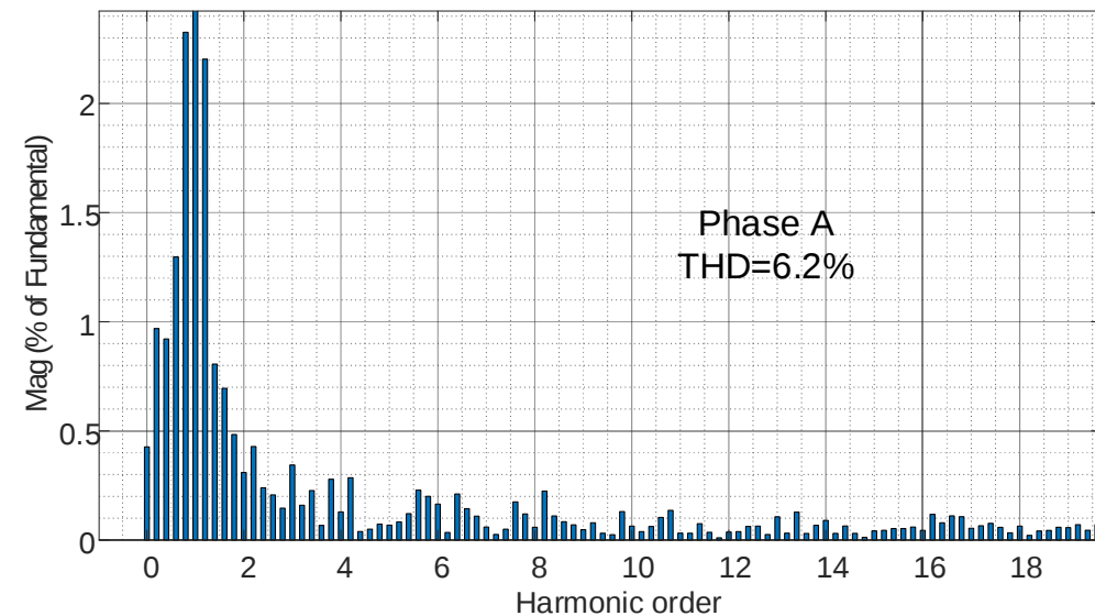
Total harmonic distortion of PI control
