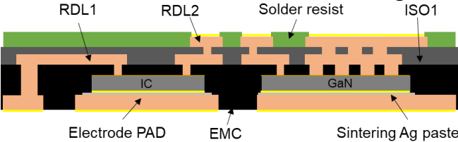
Thinner Power Module Package
