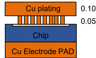
Direct Cu bonding (Without Die Attach)
