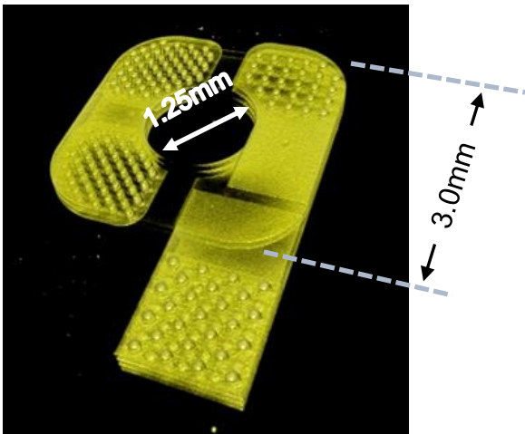
Prototype Photo & X-ray CT 3D image
