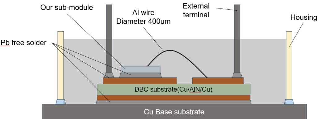
Cross-section structure
