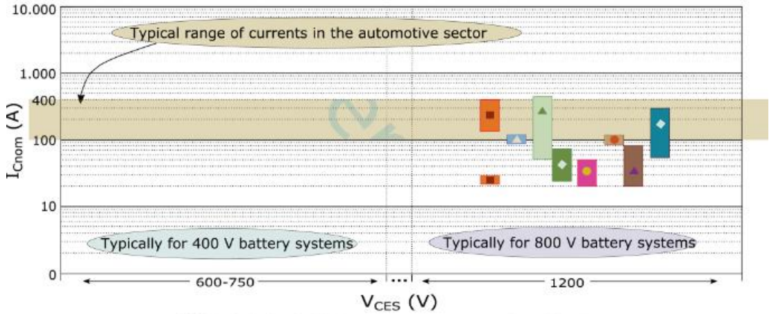
(B) Modules for the Voltage Source Inverter topology (6-in-1).
