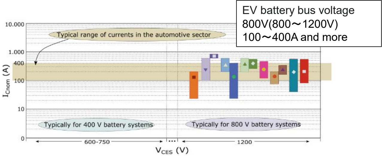
(A) Modules for the Half-Bridge topology (2-in-1).
